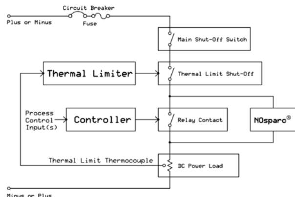
Above: detailed wiring diagram.
