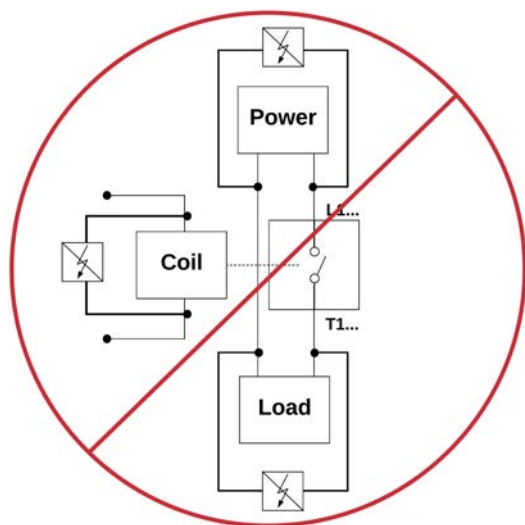
Left: IMPROPER NOsparc wiring across LOAD, across POWER, and across COIL.
