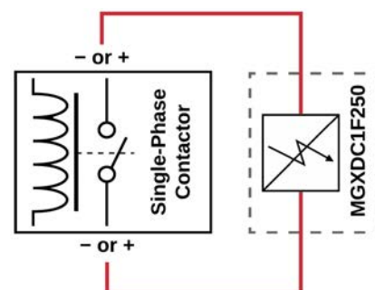
Above: simplified wiring diagram showing a NOsparc MGXDC1F250 arc suppressor connected across the contacts of a relay or contactor.
