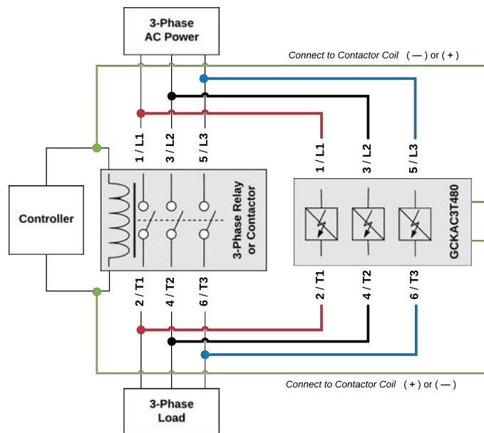
Left: Diagram contact and coil connection wiring of NOsparc GCKAC3T480 and a three-phase contactor.
