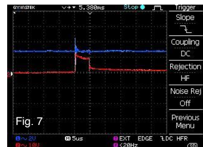
Fig. 7 is a detailed view of the initial “arclet” that triggers the arc suppressor, preventing full arc formation.
