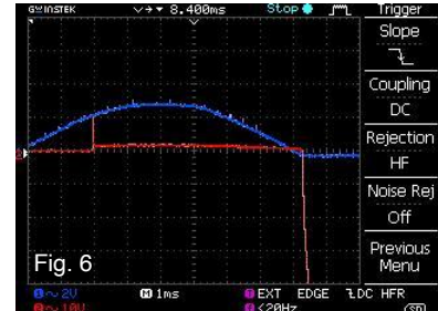
Fig. 6: With a NOsparc® electronic power contact arc suppressor across the relay contacts, the break arc is immediately suppressed and held for the 7ms until the current approaches the zero-crossing.
